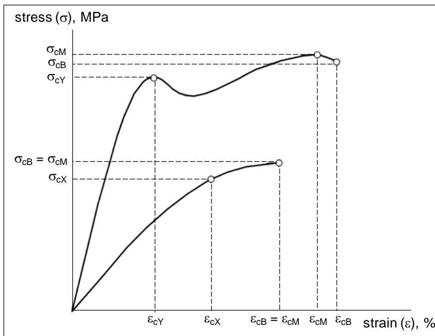
Figure 6.16 Typical compressive stress-strain curves (source: ISO 604: 2002)
