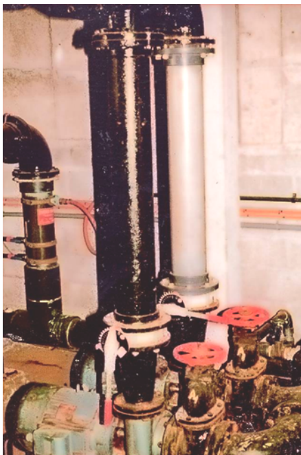
Figure 1.3 An example of metal corrosion and replacement of a length of corroded metal pipe with a plastic alternative
