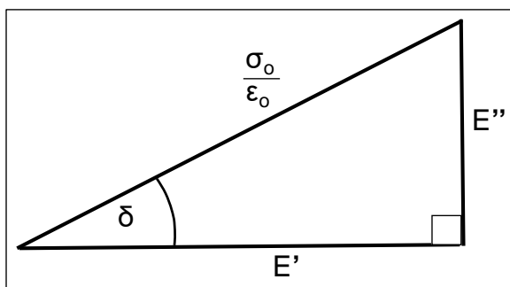
Figure 5.13 Geometric relationship between the terms E' and E''
