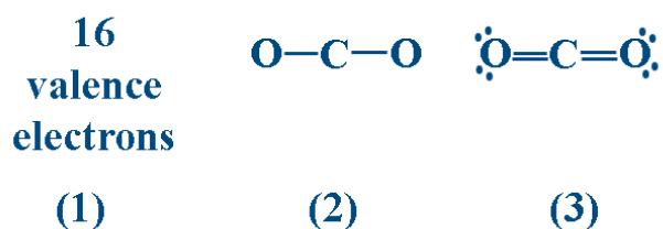
Figure 2-10: Lewis structure for the carbon dioxide molecule
