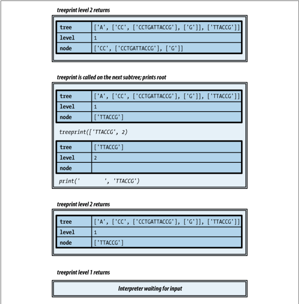
Figure 4-5. Implementation of recursion, part 3
