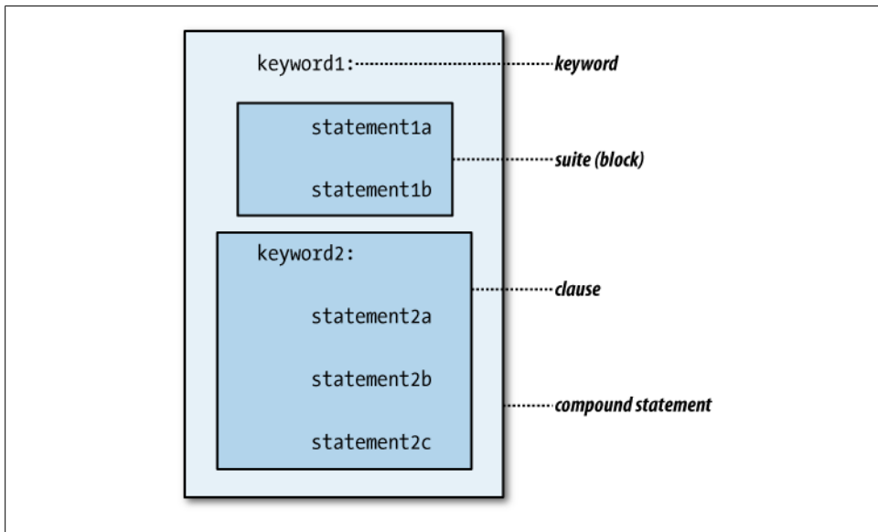
Figure 4-1. The structure of compound statements
